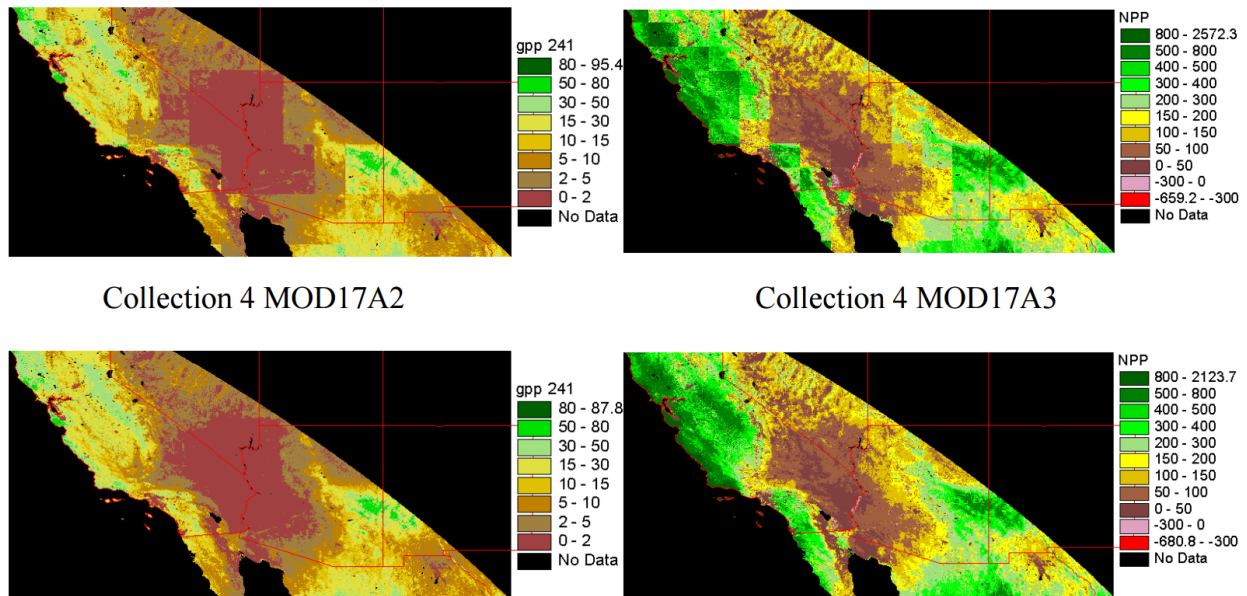
Figure 2.6. Comparison of Collection 4 and Collection 4.5 MOD17A2 GPP (composite period 241) and MOD17A3 NPP for 2001.
