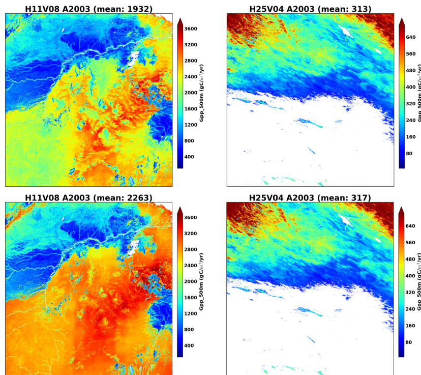
Figure 2.5. Comparisons of the annual MOD17A3H GPP from the original data (upper panel) with the year-end gap-filled (bottom panel) for two tiles. At the end of each year, MO[Y]D17A3HGF will be generated using the year-end gap-filled MO[Y]D15A2H as input. Cloudy area such as H11V08 in Amazon will be improved more than clear area H25V04 in Mongolia.
