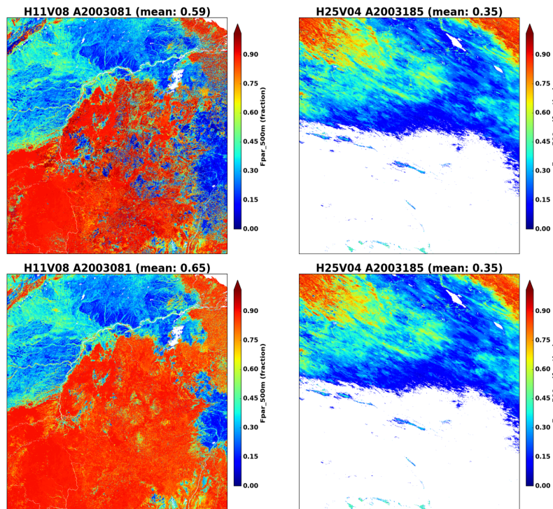
Figure 2.3. Comparisons of 8-day MOD15A2H FPAR from the original data (upper panel) with the year-end gap-filled (bottom panel) for two tiles. Cloudy area such as H11V08 in Amazon will be improved more than clear area H25V04 in Mongolia.
