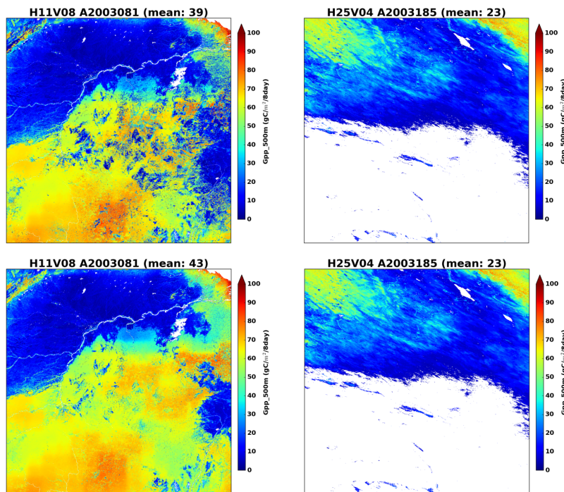
Figure 2.4. Comparisons of 8-day MOD17A2H GPP from the original data (upper panel) with the year-end gap-filled (bottom panel) for two tiles. Cloudy area such as H11V08 in Amazon will be improved more than clear area H25V04 in Mongolia.
