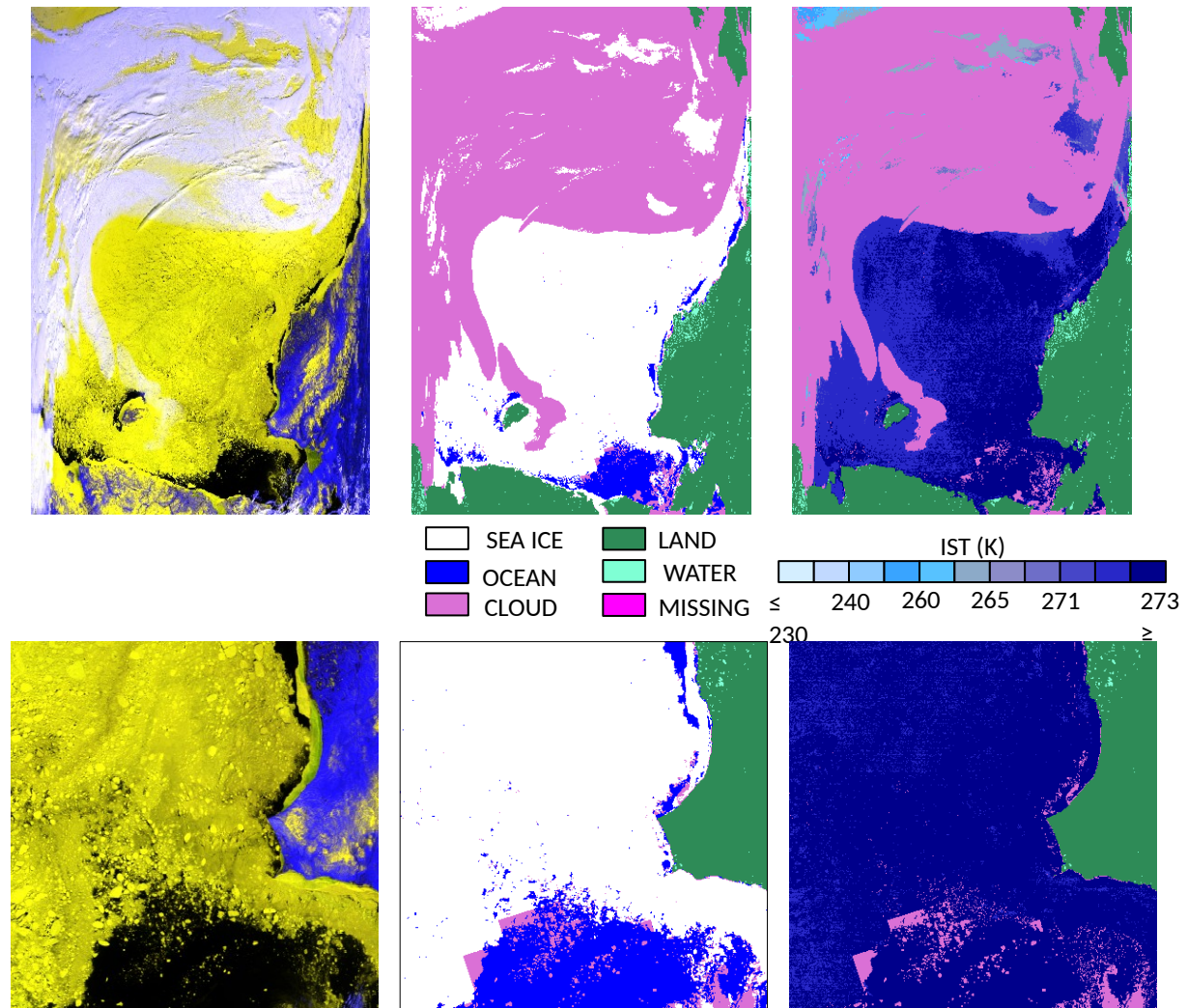
Figure 1. MOD29. A2002143.2320.006.20142320034.hdf swath product of sea ice extent (top center image) and IST (top right image) of Arctic Ocean along Alaska and Russia coasts, Seward Peninsula is located on lower right corner of image. IST scale has narrower intervals over 265-273K to show detail in that temperature range. False color (bands 1, 4, 6) image of MOD021KM.A2002143.2320.006.2014232003420.hdf shown in left image for image interpretation. At 1km resolution details of sea ice extent can be seen in clear sky conditions. Subset images in the lower row, Chukchi Sea and Lisburne Peninsula AK on right side of subset, show some detail in the data.
